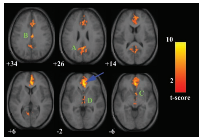
Fig. 2. Map of the resting-state neural connectivity for the vACC. The blue arrow indicates the approximate location of the vACC maximum [ 2 \ 38 \ -2 ]. A [ 2 \ -51 \ 27 ], PCC extending into the precuneus. B [ 4 \ -14 \ 34 ], rostral PCC. C [ 4 \ 9 \ -6 ], nucleus accumbens. D [ 4 \ -16 \ -3 ] is in the hypothalamus with some extension into the rostral midbrain. For other details, see Fig. 1.
