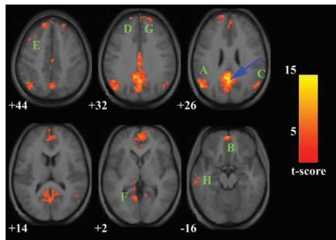
Fig. 1. Map of the resting-state neural connectivity for the PCC. The blue arrow indicates the approximate location of the PCC peak [ -2 \ -51 \ 27 ]. The approximate locations of the eight significant clusters are labeled A–H in descending order of the cluster's t score (A corresponds to the cluster with the highest t score). A [ -51 \ -65 \ 27 ], left IPC. B has a maximum at [ -2 \ 55 \ -18 ] in the OFC, but extends superiorly into the MPFC and the vACC (seen at z = +2 ). C [ 53 \ -61 \ 27 ], right IPC. D [ -16 \ 49 \ 38 ], MPFC just left of midline. E [ -44 \ 20 \ 41 ], left DLPFC. F [ -12 \ -35 \ 0 ], posterior left PHG. G [ 18 \ 54 \ 32 ], MPFC just right of midline. H [ -58 \ -18 \ -14 ], left ITC. Map is superimposed on transverse sections of the group-average structural scans. The numbers below each image refer to the z plane coordinates of Talairach and Tournoux. The left hemisphere of the brain corresponds to the left side of the image. Height and extent thresholds were set at P < 0.001 . t score scale is shown on the right.
